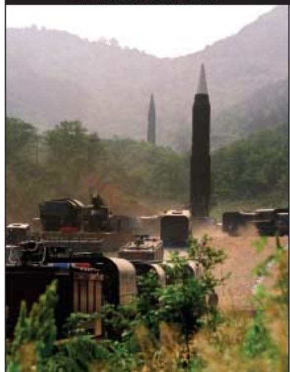
Figure 16: DF-3A (CSS-2) Twin Launch Exercise
